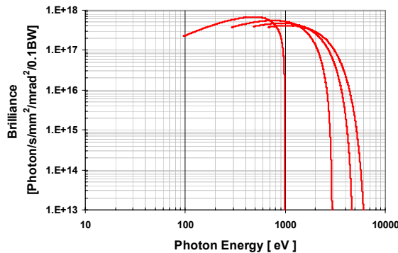
Figure 8: EPU brilliance for vertical polarization.
