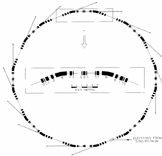
Fig-1: Layout of Indus-2
