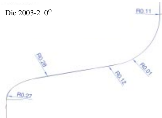
Figure 18: Shape measurement of the half-cup after removed from the die.
