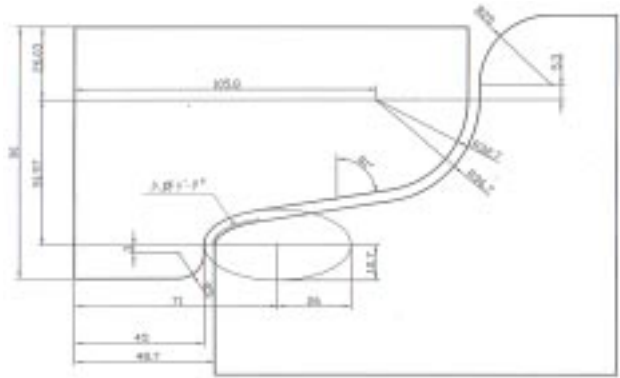
Figure 14: The set of deep drawing die (Die 2003-2).
