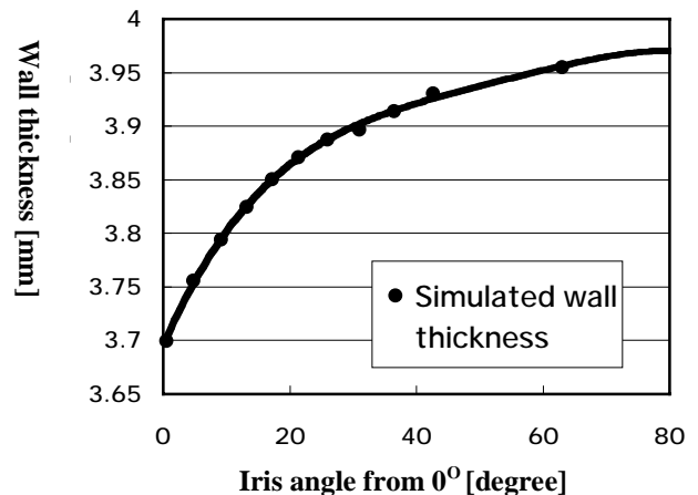
Figure 15: Estimated wall thickness at the iris section by Die 2003-1.
