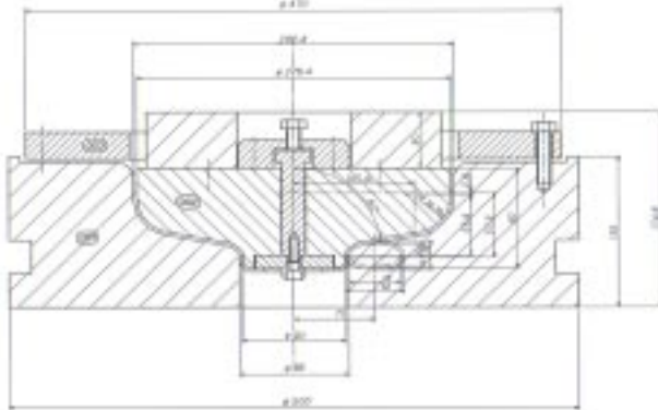
Figure 5: The set of deep drawing Die-2002.
