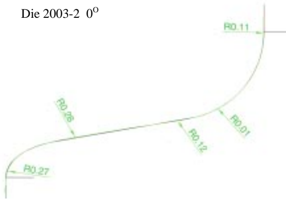
Figure 19: Shape measurement result of the half-cell in the direction of 0°.
