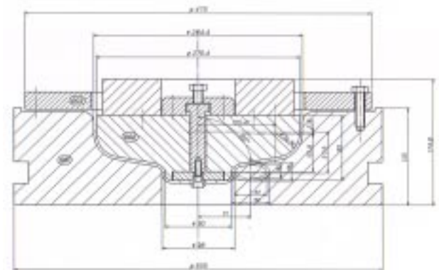
Figure 10: The set of deep drawing Die 2003-1.
