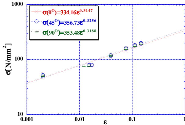
Figure 1: Measure the characteristics curve between strain and true stress.
