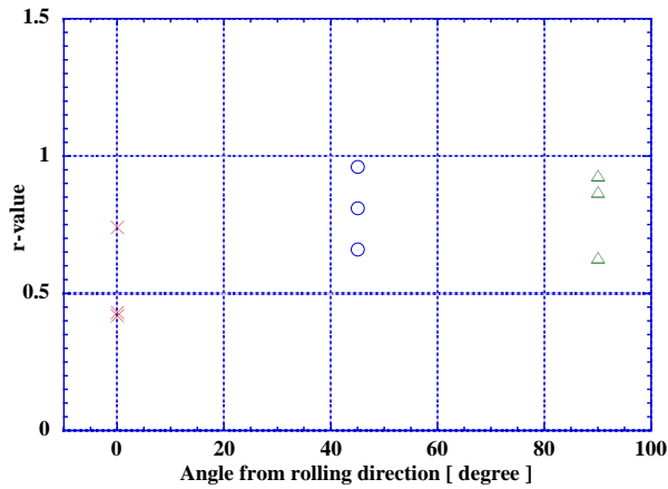
Figure 2: r-values in the three directions from the rolling direction.
