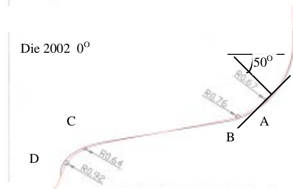
Figure 6: Simulation results with Die-2002 just on pressing.
