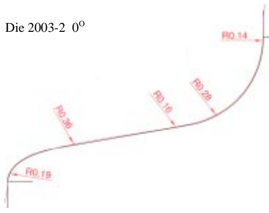
Figure 17: Simulation result for Die 2003-2 on off loading.
