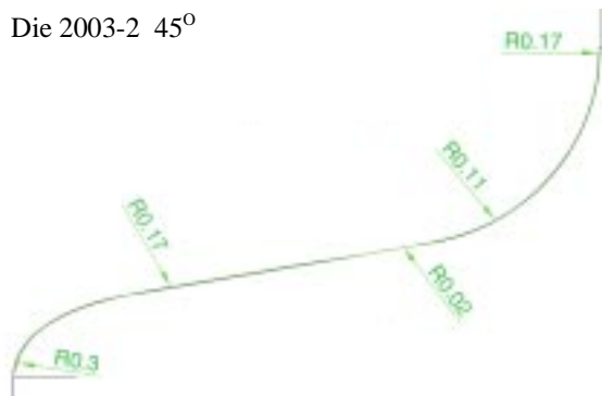
Figure 20: Shape measurement result of the half-cell in the direction of 45°.
