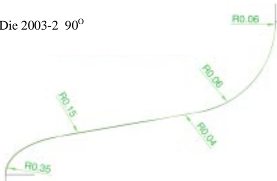
Figure 21 Shape measurement result of the half-cell in the direction of 90°.
