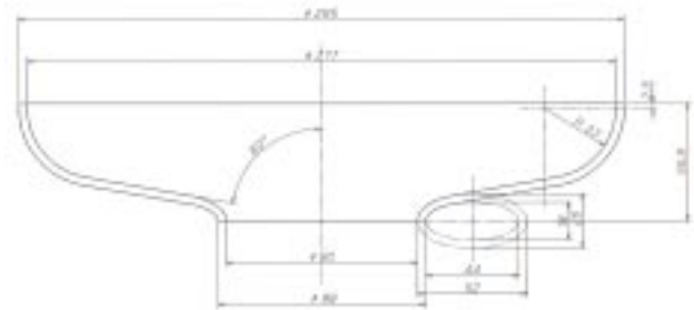
Figure 9: The designed half-cell shape for the upgraded 972MHz 9-cell structure.
