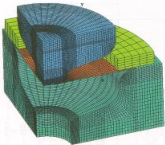
Figure 3: Meshing of the dies in the simulation.
