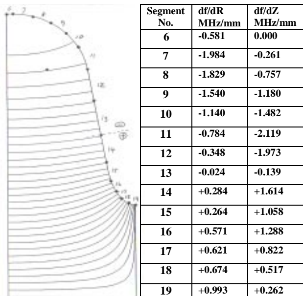
Figure 7: Simulation result with Die-2002 off pressing.
