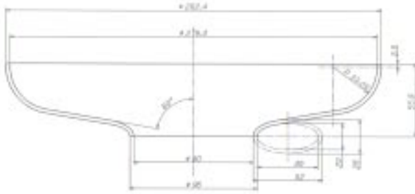
Figure 4: Half-cell design with Die-2002.
