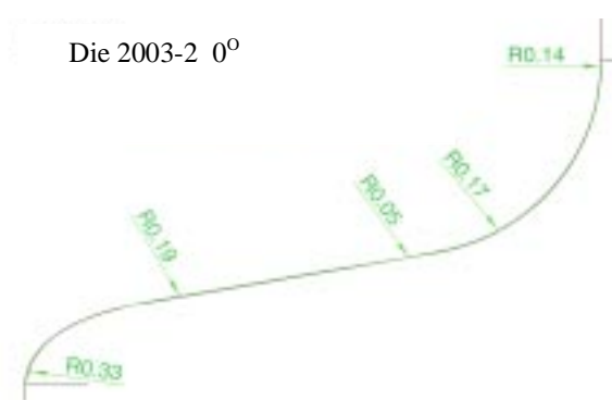
Figure 19: Shape measurement of the half-cell after trimmed.
