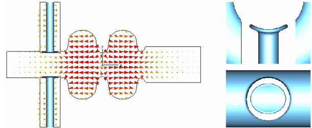
Figure 1: Geometry of the cavity with the fundamental mode excited in it and details of the coupler.
