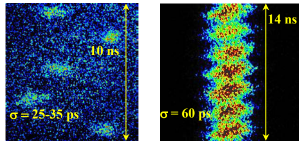
Fig. 4: On the left, unstable beam when the cavity is parked, on the right stable beam when the cavity is active.
