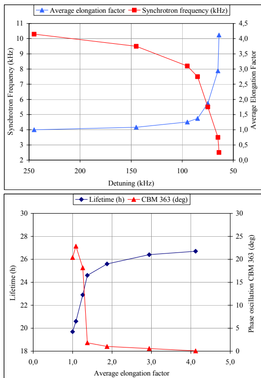
Fig. 2: Lifetime and CBM 363 vs the elongation factor.
