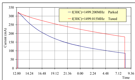
Fig. 3: Beam current decay with SUPER-3HC active (red) and parked (blue).
