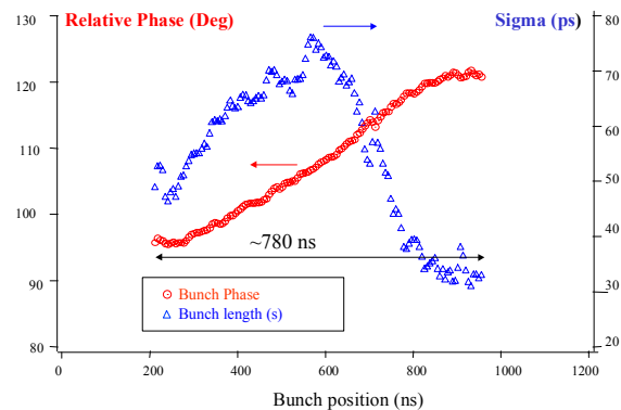
Fig. 5: Phase Modulation along the bunch train.
