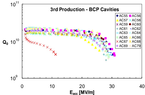
Figure 1: Excitation curves of all cavities of the third production series treated with BCP. The measurements were done in a vertical test cryostat at 2 K.
