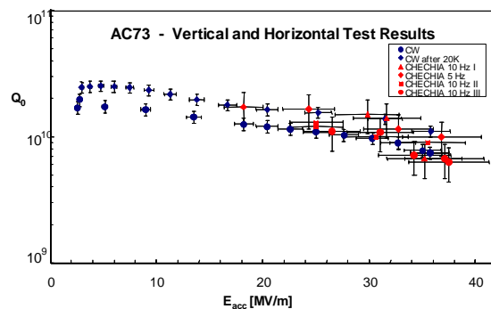
Figure 3: Excitation curves of the electro-polished high-performance 9-cell TESLA cavity AC73 in vertical (cw) as well as horizontal (CHECHIA) tests. The systematic rms errors in the determination of the accelerating field and the quality factor are indicated.
