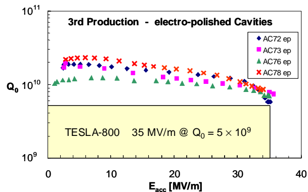
Figure 2: Excitation curve of high-performance 9-cell TESLA cavities treated with EP. The cavities are cooled by superfluid helium at 2 K.
