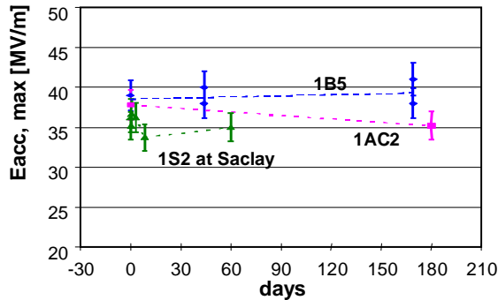
Figure 4: Development of cavity gradient after storage under clean room air.
