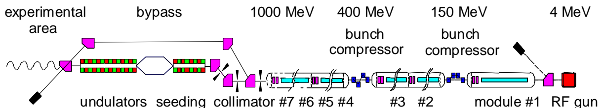
Figure 5: Schematic layout of the superconducting TTF linac for phase II. The electron beam direction in this picture is from right to left.
