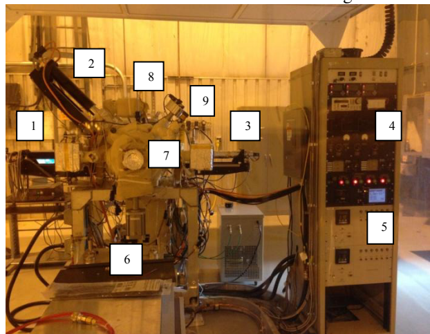
Figure 1: The picture of ERL-deposition system: 1 – K source; 2 – Sb source; 3 – Cs source; 4 – control system for valves and source; 5 – power supply for baking; 6 – table for supporting cathode transport cart; 7 – load lock port; 8 – heater; 9 – crystal monitor.
