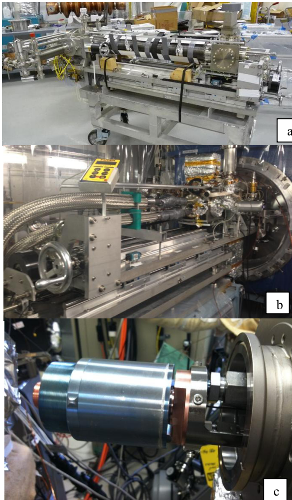
Figure 2: Photographs of the cathode and transport cart: a) The cathode transport cart; b) The transport cart attached to the gun and the cathode stalk inserted. Two line attached to the manipulator are for cooling the cathode in the gun. Same port will be used for heating the substrate during cathode preparation; c) The cathode stalk mounted on the transport cart.
