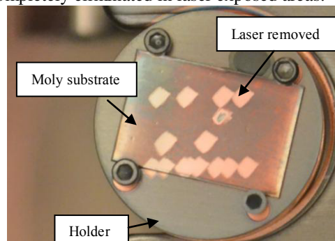
Figure 4: Excimer laser radiated K 2 CsSb cathode sample. The rectangular regions are exposed to the laser. The cathode material in these regions is removed.
