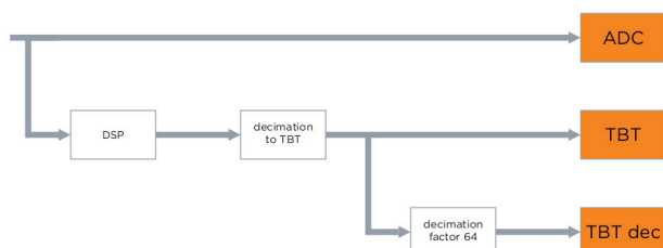
Figure 3: Data-paths and buffers overview.
