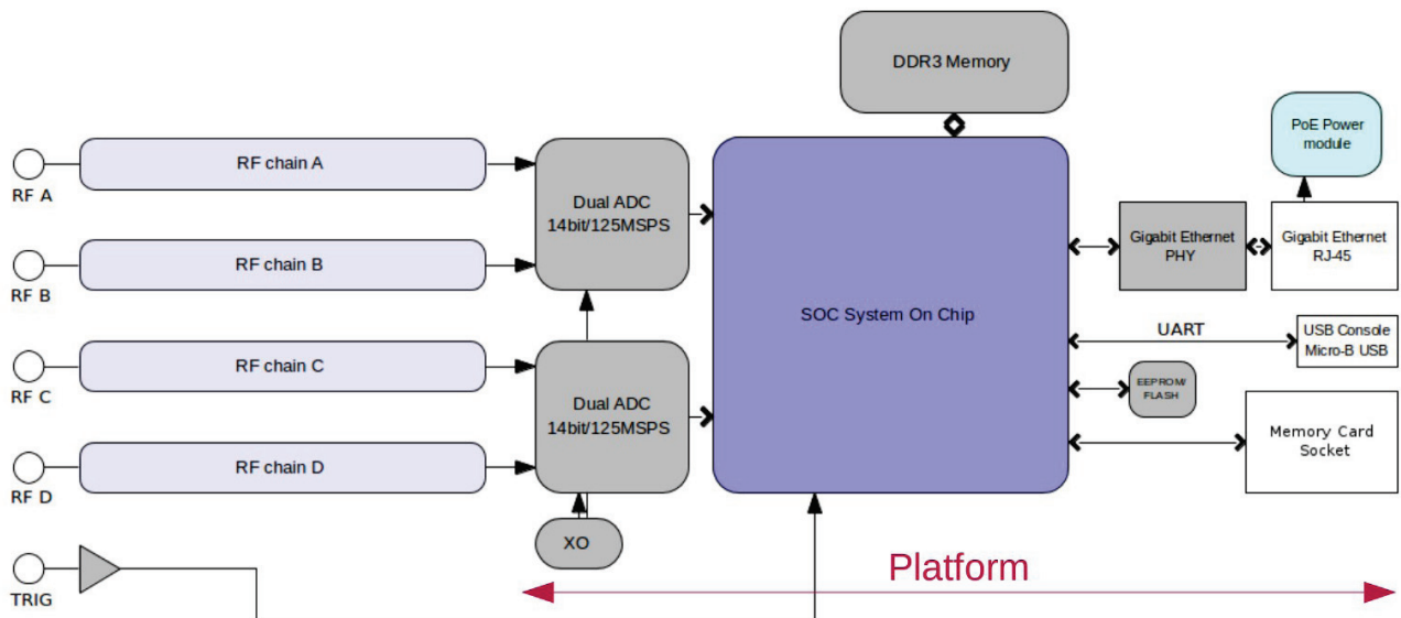
Figure 2: Basic HW architecture of the BPM instrument.
