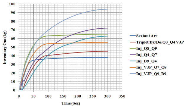
Figure 3: Helium inventory loss.
