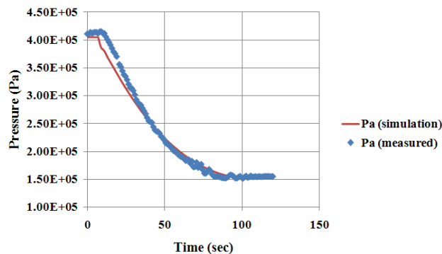
Figure 5: RHIC sextant depressurization test results.
