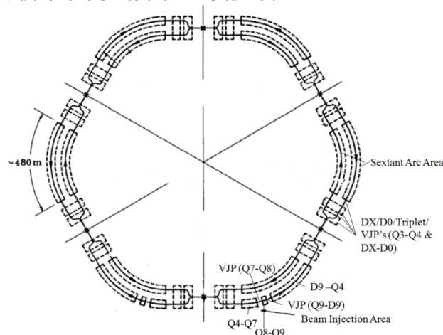
Figure 1: RHIC rings and three typical areas.
