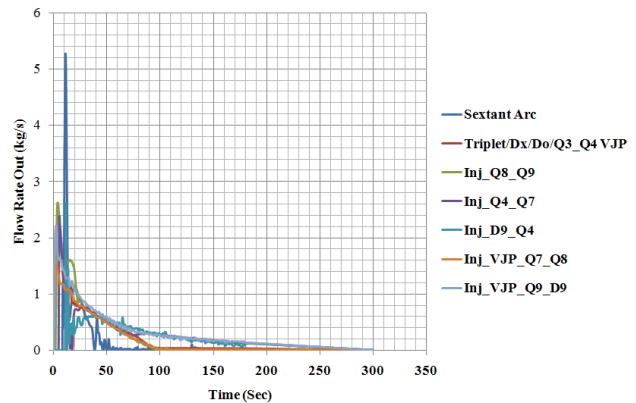
Figure 2: Helium release rates out of relief valves.
