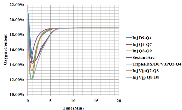
Figure 4: Oxygen content in RHIC tunnel near the helium discharge location.
