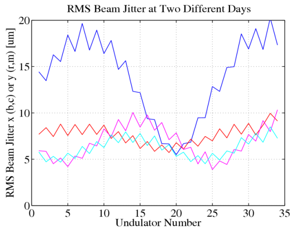
Figure 7: The RMS jitter is plotted versus undulator position for two different days (blue and cyan for x , red and magenta for y ).
