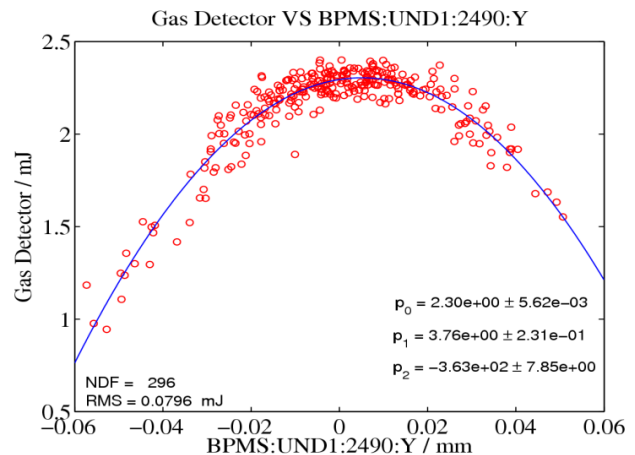
Figure 6: FEL intensity (mJ) versus Undulator y position, beam energy was 6.71 GeV. Any orbit variation outside of \pm 15 \mu\text{m} (or > 5 \mu\text{m} rms) causes a reduced FEL intensity.
