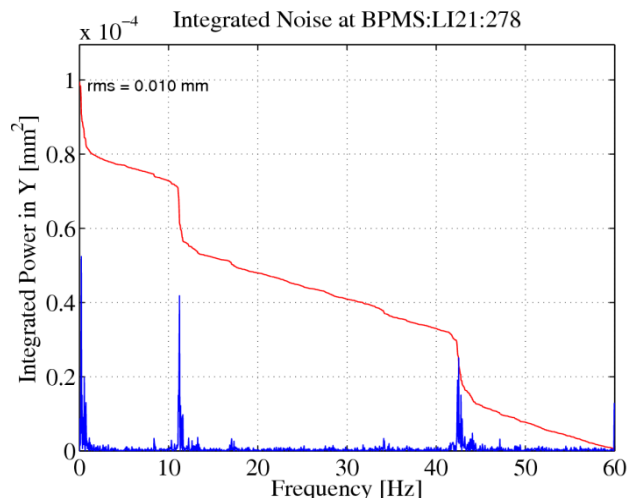
Figure 1: Power (blue) spectrum and integrated power (red) for a BPM in y in the LCLS Linac indicating 55% of the jitter power is coming from lines at 1, 11 and 42 Hz.
