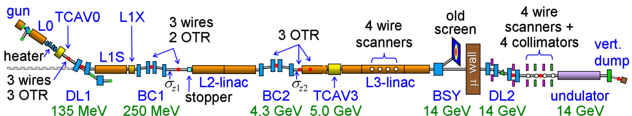
Figure 5: LCLS schematic layout of the Linac sections (L0, L1, L2, and L3) with the two bunch compressors (BC), followed by a dog leg (DL2) and some collimation before reaching the undulator and dump.
