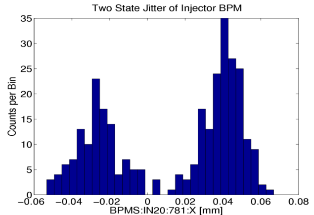
Figure 4: Two-state random jitter was finally tracked down as transverse RF kicks at the L0A load.
