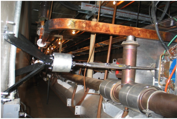
Figure 3: Wall strut for suppressing horizontal motion of a quadrupole.
