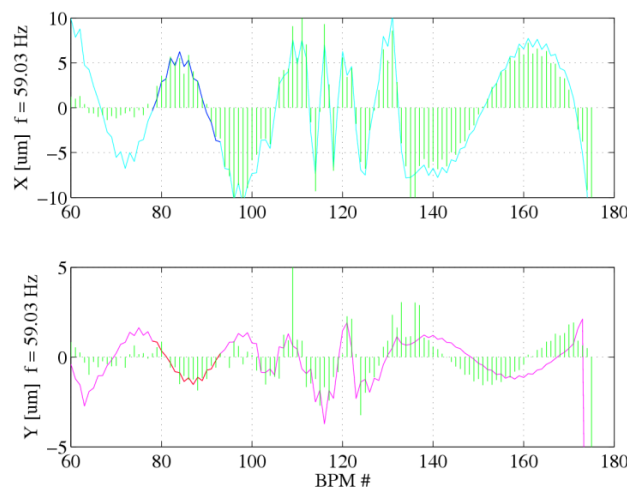
Figure 2: The 59 Hz component (mainly in x ) generated by Linac accelerator pumps can be located here to the 5 th quadrupole in Sector 28 in x and the 8 th in y .
