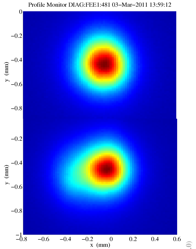
Figure 8: FEL spots on a YAG screen (Direct Imager), top with laser heater on bottom with it off at 150 pC charge.
