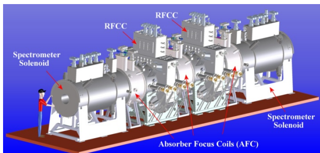
Figure 1: The MICE cooling channel.
