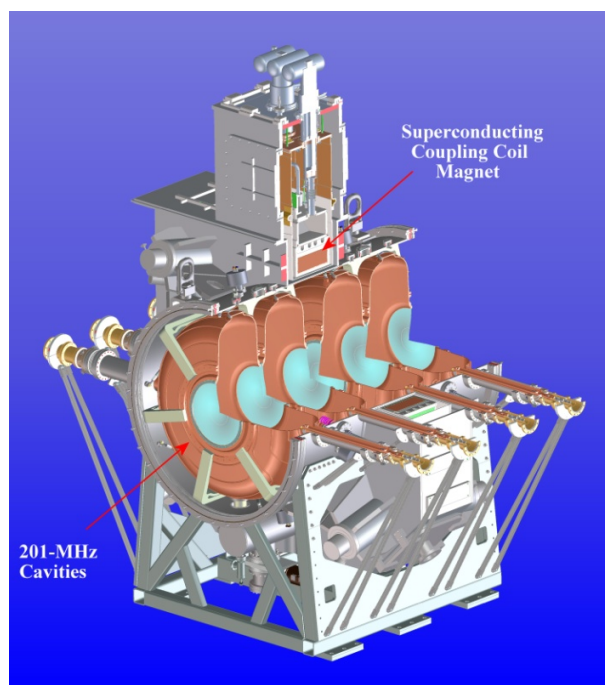
Figure 2: 90° sectioned view of the MICE cooling channel RFCC module.
