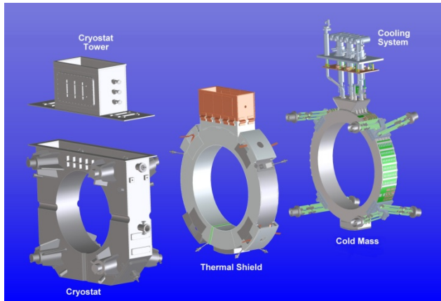
Figure 4: Components of the superconducting coupling coil magnet.
