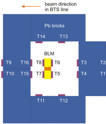
Figure 1: Plan view of TLD placement on the BLM and Pb shield.
