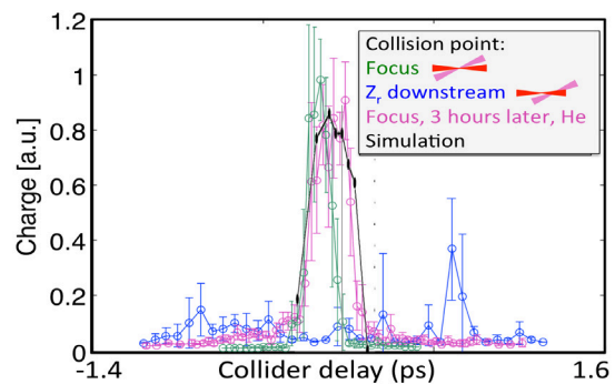
Figure 3: Scan of the collider timing with respect to the driver shows a 200 fs window of overlap region where injection is optimized. Charge stability is \sim 20\% . The experimental result agrees well with simulations (which were conducted with a_1 = 0.5 ). Charge versus timing for two different intersection points between driver and collider shows that charge falls off rapidly for intersection \sim Z_R after focus. Performance is repeatable hours later and similar in He and H gas jets.
