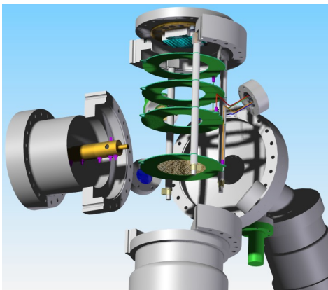
Figure 4: Experimental chamber and extraction system for the density mapping of the supersonic-jet curtain.
