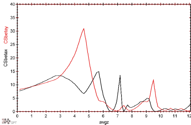
Figure 7: \beta_{x,y} for the tomography section of the ALICE to EMMA injection line from GPT at 35 MeV and 80 pC, following correction for space charge.
