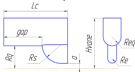
Figure 5: Basic dimensions of improved vanes.
