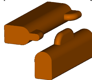
Figure 4: Adjacent vanes with improved profile.
