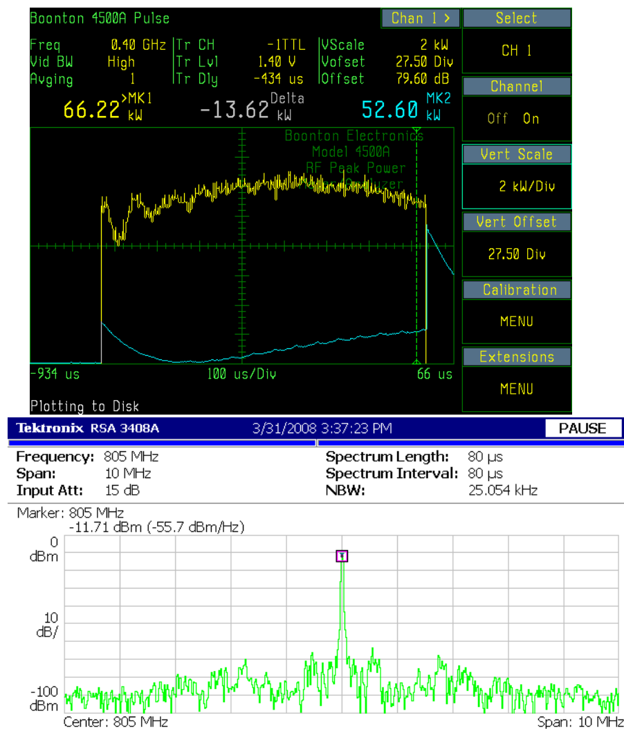
23b Cavity input full power parabolic shape
