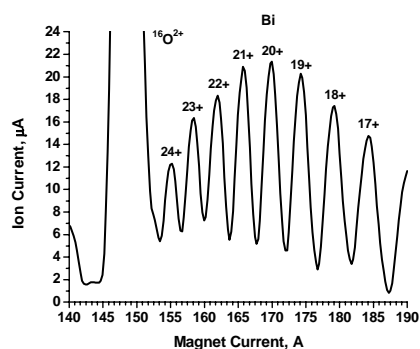
Figure 2: Bismuth beam intensities for different charge states.
