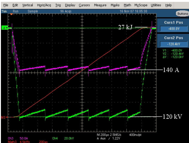
Figure 4: Marx output with coarse flattening, Ch3 is load current, Ch4 is load voltage, and Math3 is load energy.
