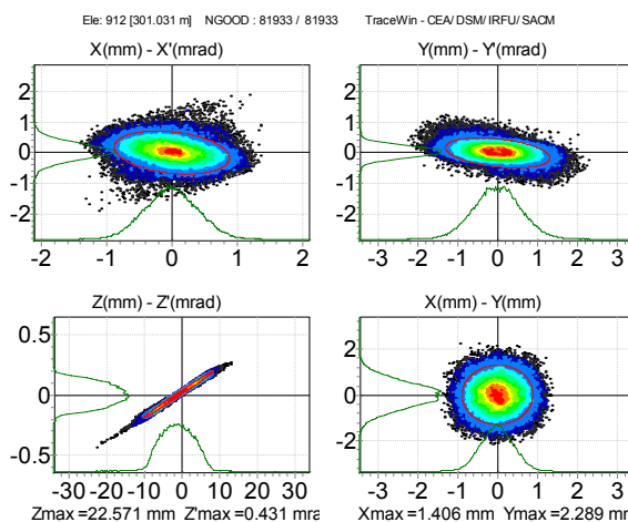
Figure 5: Proton beam at target in the phase spaces.
