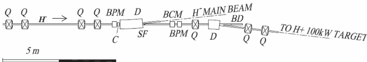
Figure 3: CW beam splitter layout (1 section). The main H - beam (coming from left) is partially neutralized in a small magnetic chicane (C). In the first bending magnet (D), the main H - beam is guided to the next splitter section, while the H 0 particles move straight to the stripper foil (SF), to be stripped into H + and then transported to the target. Q=quadrupole magnet; BD=beam dump; BCM=beam current monitor; BPM=beam profile monitor.
