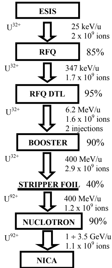
Figure 1: Injection chain of the NICA collider based on ESIS source and RFQ linac.
