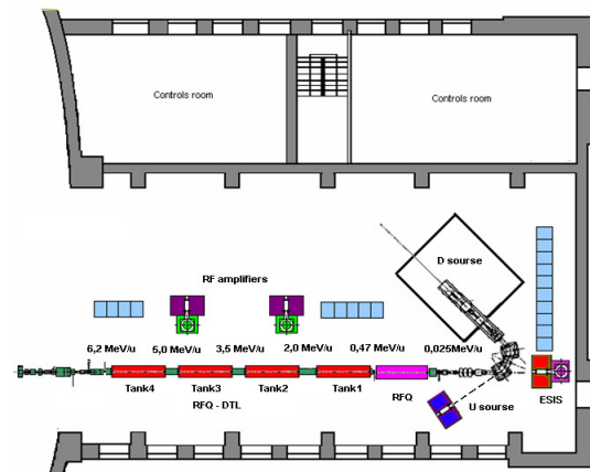
Figure 2: Injector location in the existing building.
