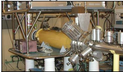
Figure 3: ESIS "KRION-2" operated at JINR.
