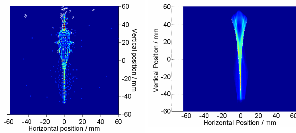
Figure 1: Left, simulated and right, measured beam profile.
