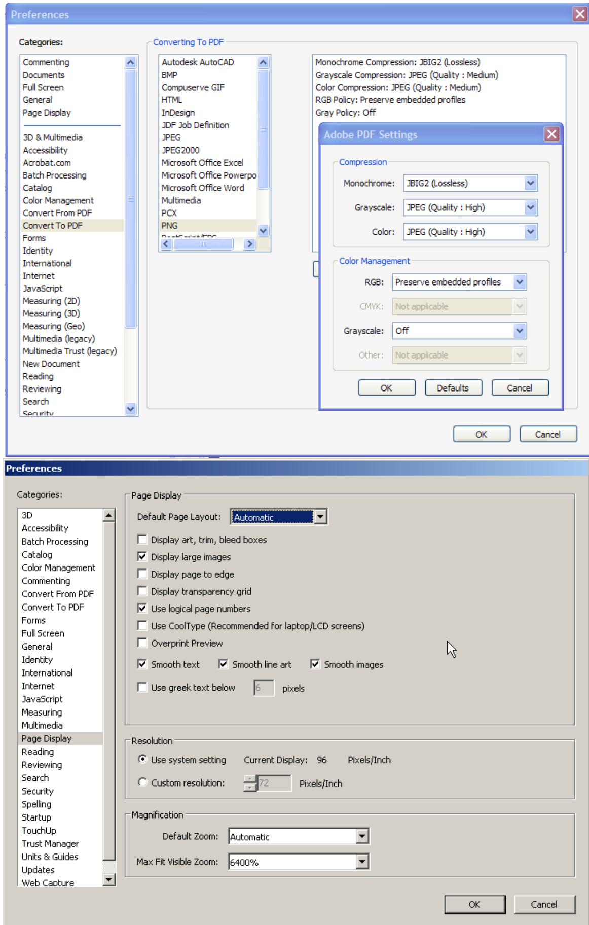
Figure 8: Page Display Window of the Preferences Setup
