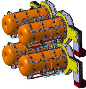
Figure 2: Horn layout (the targets are inside the horns).
