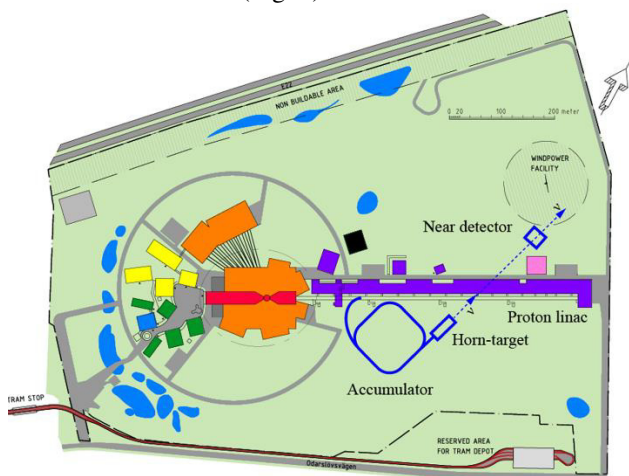
Figure 1: ESSvSB layout on top of the ESS neutron facility.
