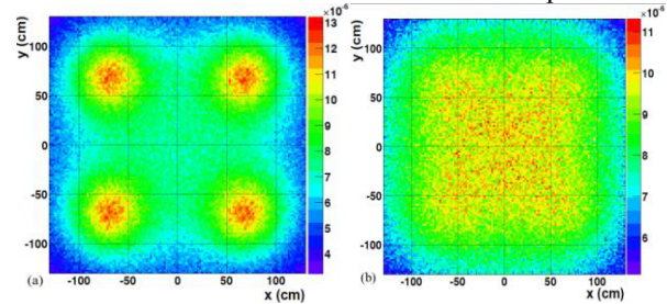
Figure 3: Pions (a) and muons (b) at the surface of the beam dump (normalized by proton).
