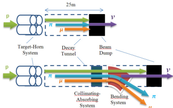
Figure 5: Principle of muon extraction.
