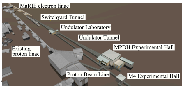
Figure 1: The MaRIE Facility layout.
