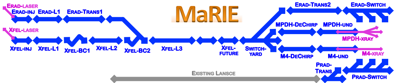
Figure 2: The MaRIE beamline layout.
