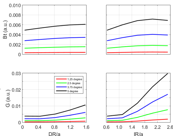
Figure 3: B_t (top) and G (bottom) as function of DR/a (left) and IR/a (right) for the yaw tilt case.
