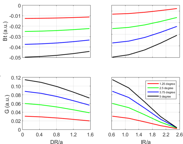
Figure 2: B_t (top) and G (bottom) as function of DR/a (left) and IR/a (right) for the pitch tilt case.
