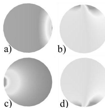
Figure 5: Dipole field from a single helical wire placed at a) 0 degrees, b) 90 degrees, c) 180 degrees, and d) 270 degrees.
