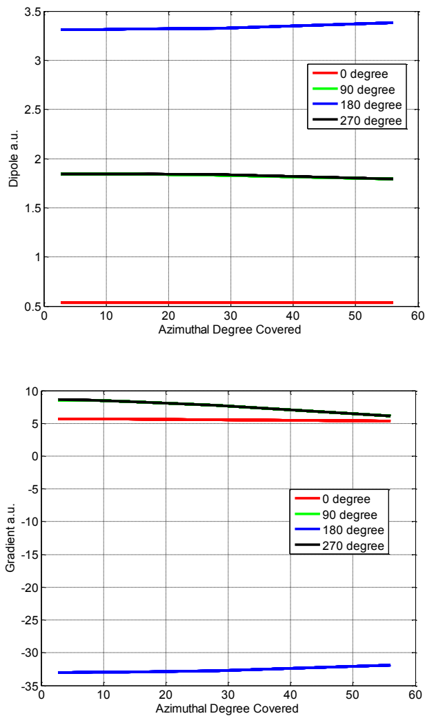
Figure 6: Dipole (top) and Gradient (bottom) produced by the addition of helical lines on the inner bore.
