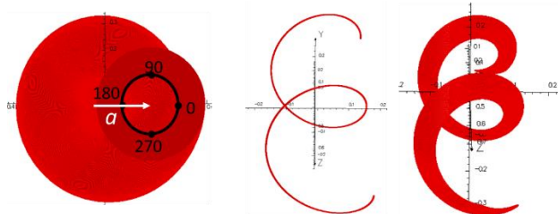
Figure 4: End view of the helical cooling channel showing the four positions for the added helical lines (left). An example of a single helical line and twenty lines (right).
