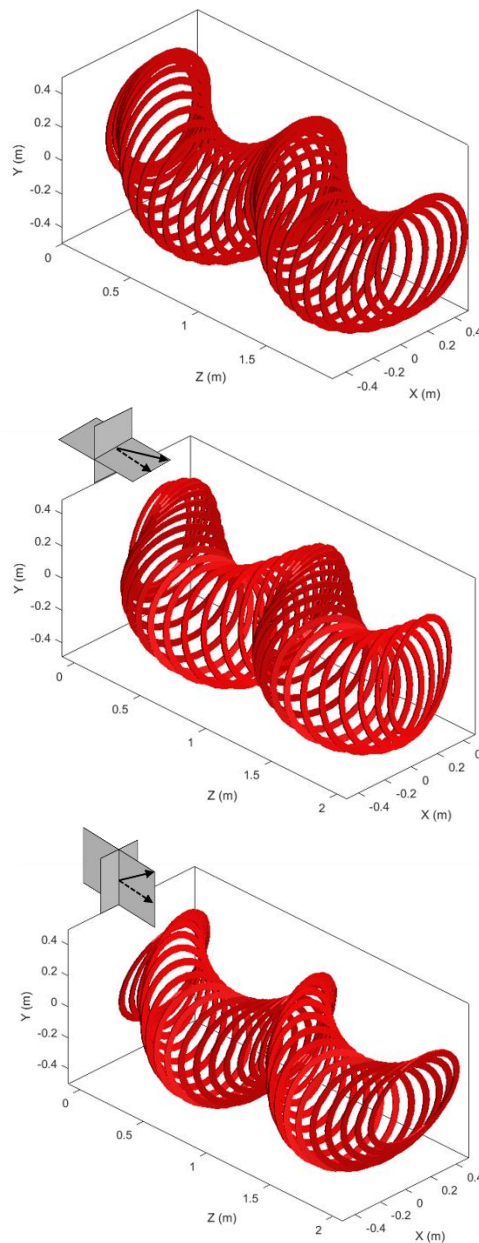
Figure 1: Helical coil arrangement of the non-tilted coil (top), Yaw tilt (middle), and Pitch tilt (bottom). The spacing between the coils and tilt were exaggerated for clarity.
