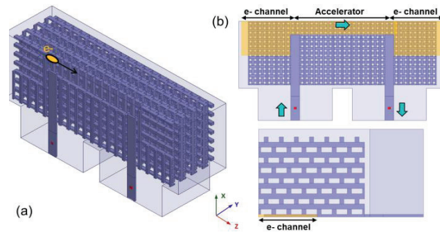
Figure 4: (a) Schematic of a fully forward coupled silicon woodpile accelerator, and (b) its bottom view and side view highlighting its open sections as electron channels and accelerating waveguide.
