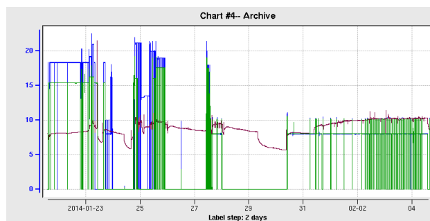
Figure 1: Showing Beamline Vacuum level in C100-10 cryomodule when gradients were lowered to 10 MV/m (Dark Red is the Beamline vacuum, Blue and Green are gradients in Cavity 6 and 7)
