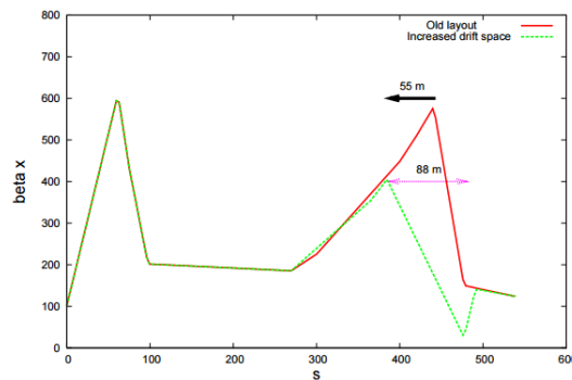
Figure 2: Horizontal \beta -function for rearranged optics to accommodate both extraction and crossing in IR1.
