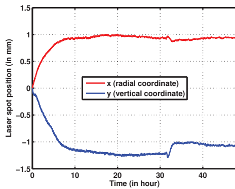
Figure 4: Laser spot position with respect to time when laser beam propagates over 35 m in vacuum.
