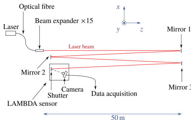
Figure 1: Schematic top view of the setup in air.
