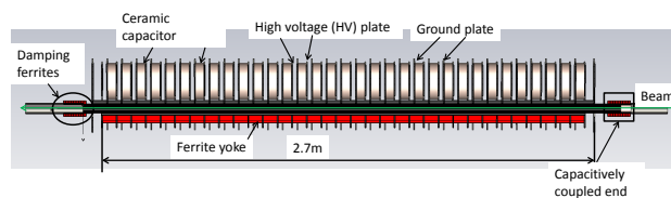
Figure 1: Structure of the injection kicker magnets.
