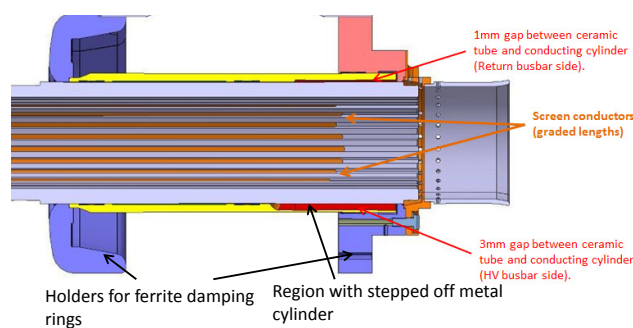
Figure 2: Cross section of the new beam screen design.
