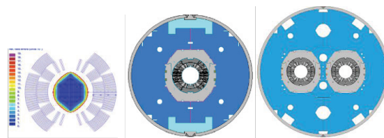
Figure 6: The 2-layer coil (left), single aperture (middle) and twin-aperture (right) dipole cold masses. The dark area in the coil corresponds to relative field errors below 10 -4 .
