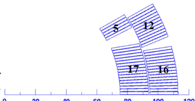
Figure 3: Octant of the QXF quadrupole coil. The number of cables in each block is also indicated.
