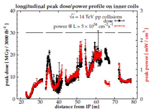
Figure 2: Heat deposition in the coil (left scale) and radiation damage (right scale) for 150 mm aperture triplet.
