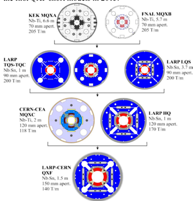
Figure 4: Overview of low-β quadrupole developments.
