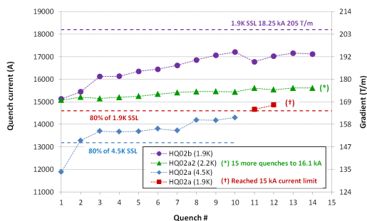
Figure 5: Quench performance of HQ02, reaching 95% of the Short Sample Limit.
