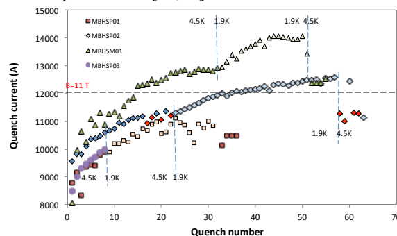
Figure 7: Summary of 11 T magnets trainings.
