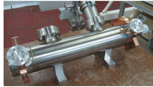
Figure 4: Assembled PETS and leak test.
