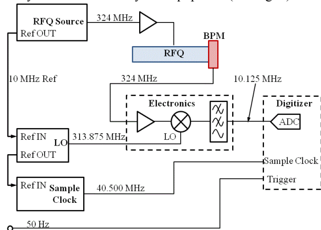
Figure 4: BPM clock reference (one electrode processing channel shown).
