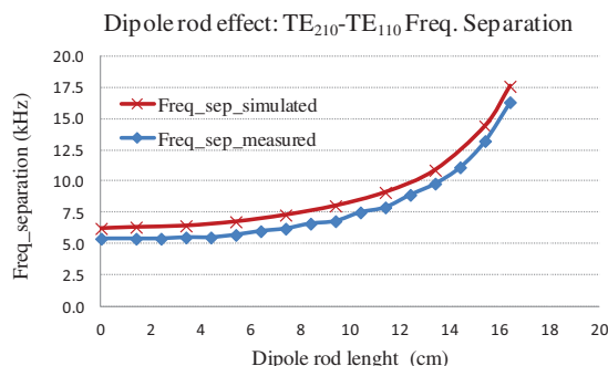
Figure 5: Dipole stabilizer rods effect.
