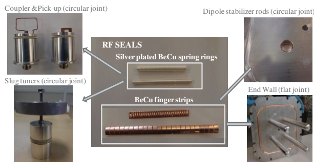
Figure 3: RF seals tested including dipole rods.
