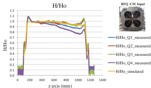
Figure 7: Magnetic field normalized profile.
