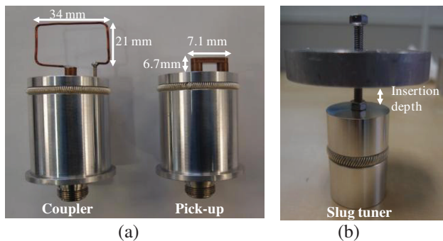
Figure 2: (a) Coupler and pick-up; (b) slug tuner.
