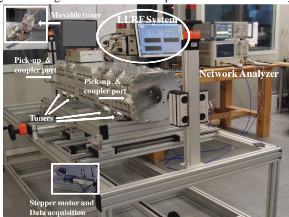
Figure 1: RFQ-CM measurement test-bench.
