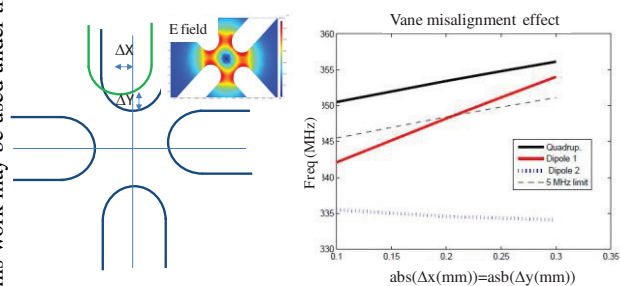
Figure 6: Vane misalignment study.
