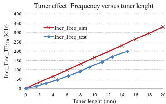
Figure 4: Frequency tuning range per tuner.
