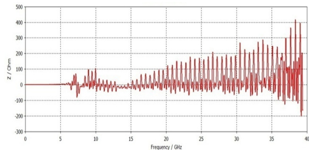
Figure 4: The longitudinal impedance of final optimized case, higher order modes are excited up to 40 GHz.
