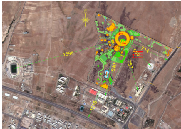
Figure 3: Satellite photo of vibration sources distances from main building of ILSF.
