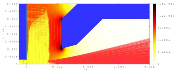
Figure 7: The electric field strength, equipotential field lines (green), H^- ion trajectories (red), and electron trajectories (yellow) for a 2.1 mm extraction electrode jaw gap.
