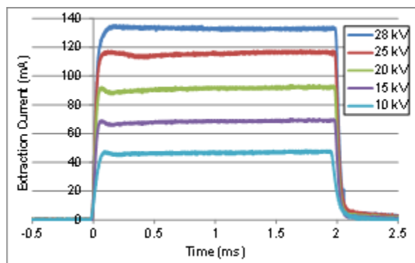
Figure 4: Extraction power supply currents, 2 ms, 50 Hz duty cycle into a 215 kΩ resistive load.
