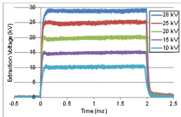
Figure 3: Extraction power supply voltages at a 2 ms, 50 Hz duty cycle into a 215 kΩ resistive load.
