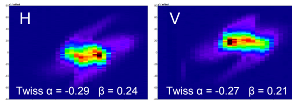
Figure 5: Emittance and beam currents for a 2.1 mm wide extraction jaw gap.
