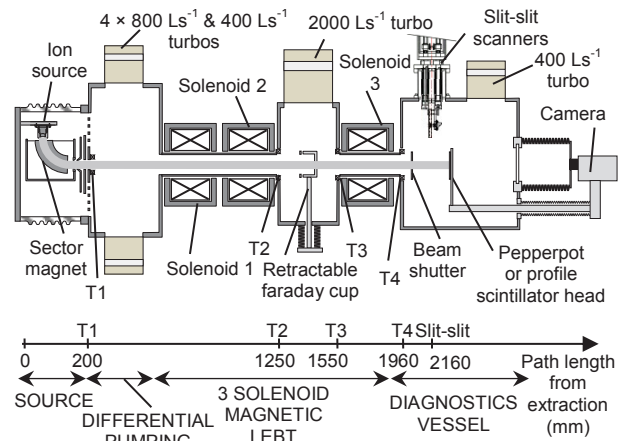
Figure 2: The FETS ion source and LEBT schematic.
