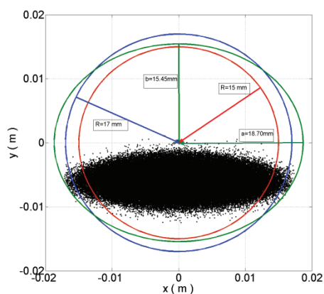
Figure 2: Cavity bore geometry scenarios for FETS MEBT.
