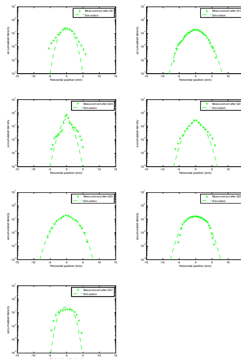
Figure 5: The measured and simulated mismatched beam profiles in 60^\circ FODO channel.
