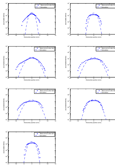
Figure 4: The measured and simulated mismatched beam profiles in 45^\circ FODO channel.
