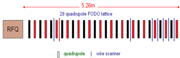
Figure 1: Block diagram of beam halo experiment transport line.
