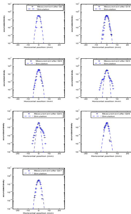
Figure 2: The measured and simulated matched beam profiles in 45^\circ FODO channel.
