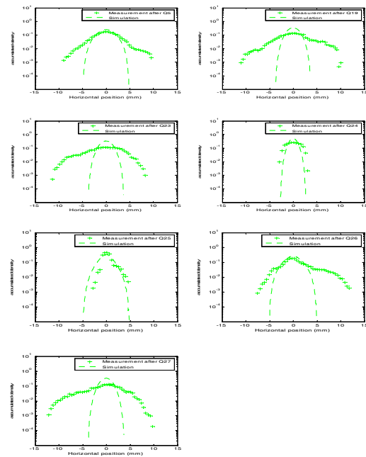
Figure 7: The measured and TraceWin simulated mismatched beam profiles in 90^\circ FODO channel.
