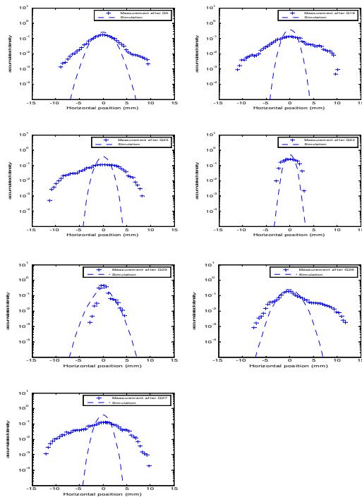
Figure 6: The measured and IMPACT simulated mismatched beam profiles in 90^\circ FODO channel.
