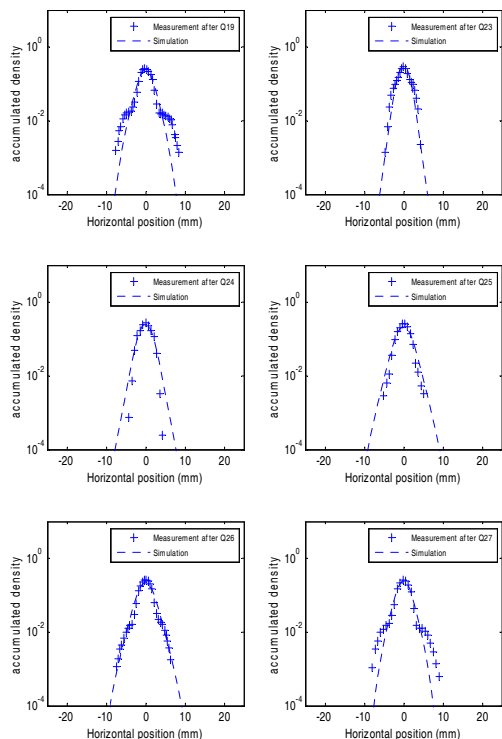
Figure 3: The measured and simulated matched beam profiles in 45^\circ FODO channel.
