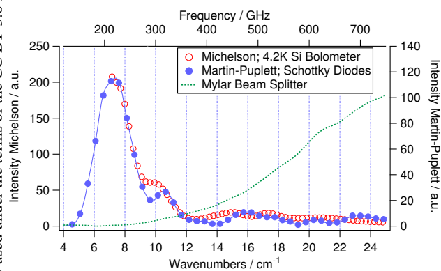
Figure 5: Spectra taken with Michelson and Martin-Puplett interferometer at the same beamline and machine settings. Both have been normalized by the beam splitter respective detector response function.
