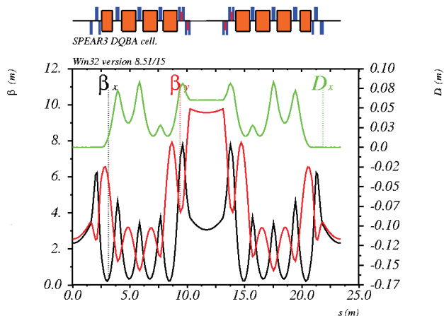
Figure 2: Optics function of SPEAR3 DQBA cell.
