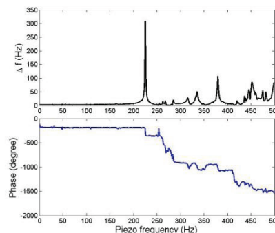
Figure 5: Piezo tuner to cavity detuning transfer function.
