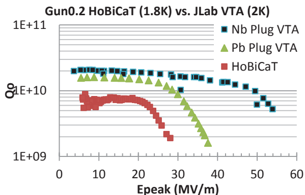
Figure 4: The Q vs. E_{peak} curve of Gun0.2 taken in HoBiCaT at 1.8 K compared to the data from the JLab VTA at 2K.
