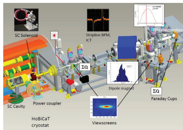
Figure 1: An overview of the SRF injector in HoBiCaT (left) connected to the diagnostic beamline.
