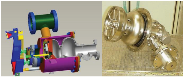
Figure 2: A model of the 1.6 cell Pb/Nb plug gun with the helium vessel and tuner alongside a picture of the cavity with the cold part of a TTF-III input coupler attached.
