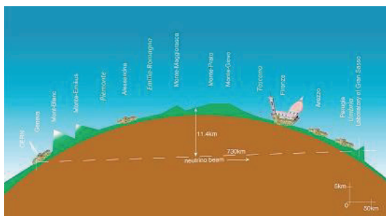
Figure 1: Schematic profile of the neutrino path.
