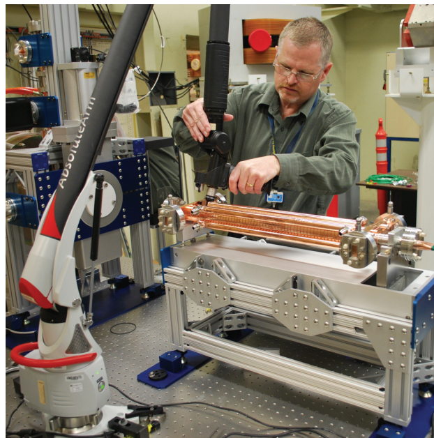
Figure 3: Photograph of X-band test station alignment. Romer CMM arm in use to precisely measure the 3D position of the T53 cells for proper alignment of the accelerating structure with respect to the beamline axis and cathode position.
