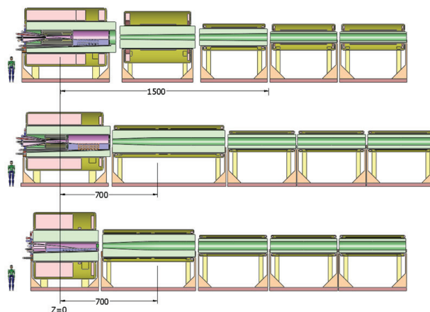
Figure 2: Vertical sections of Target-System magnet configurations with 20 T (top, middle) or 15 T (bottom) at the target, which ramp the magnetic field down to 1.5 T over 15 m (top) or 7 m (middle, bottom).
