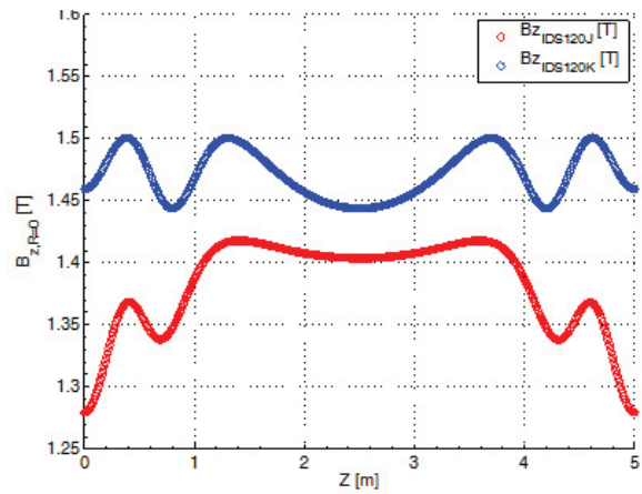
Figure 5: Axial magnetic field profiles for the 5-m-long modules of the IDS120j (red) and ISD120k (blue) configurations.
