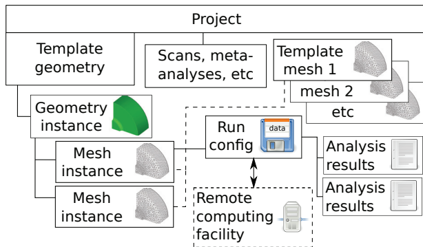
Figure 2: Data structure in an AcOpti project.
