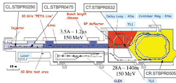
Figure 1: Layout of CTF3 and position of available phase monitors.
