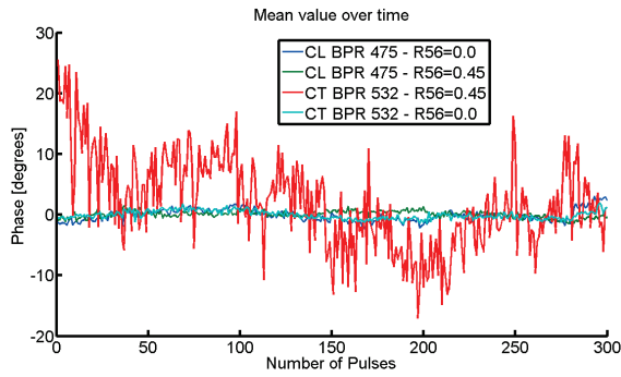
Figure 5: Mean pulse value vs. time for two BPRs (one positioned before the chicane and the other after) for R56=0.0 and R56=0.45.
