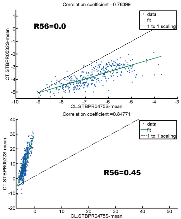
Figure 7: Correlation between BPRs 475 and 532 for different values of R56.
