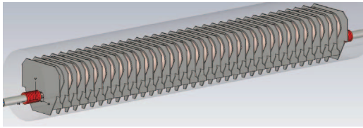
Figure 3: Schematic of the MKI. The tank is shown transparent, the red tiles are the damping ferrites, and the internal magnet structure can be seen.
