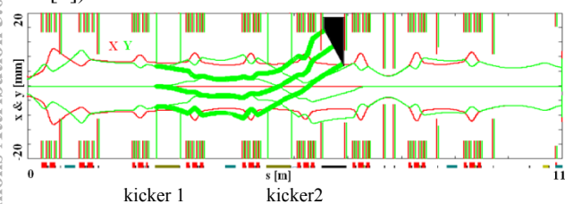
Figure 1: Scheme of MEBT optics [4] and the beam envelope. The thin lines are the central trajectory and 3\sigma envelope of the passing beam, and the thick lines are the Y envelope of the chopped-out beam.
